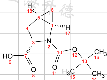
(1R,3S,5R)-2-(tert-Butoxycarbonyl)-2-azabicyclo[3.1.0]hexane-3-carboxylic acid
