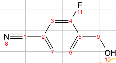
3-Fluoro-4-(hydroxymethyl)benzonitrile CAS:219873-06-0
